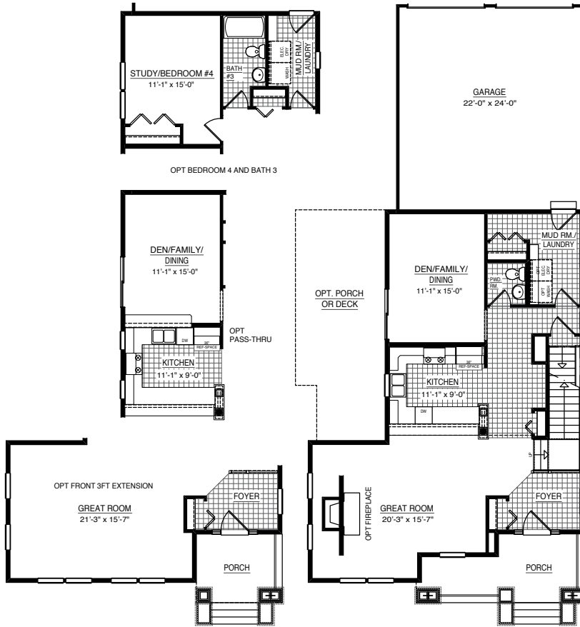
MAIN LEVEL
