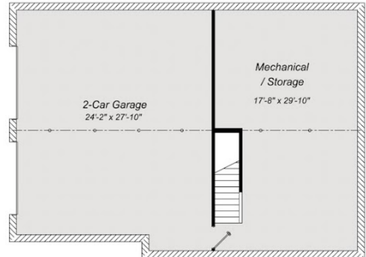
Basement Plan
